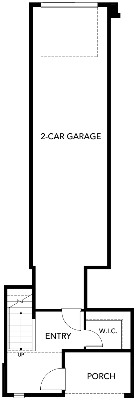
FIRST FLOOR
